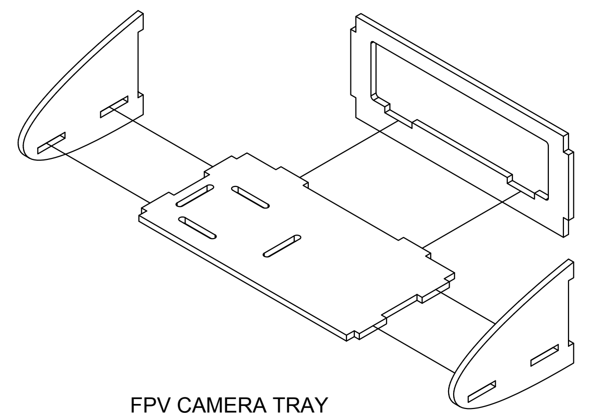
FPV CAMERA TRAY EXPLODED ASSEMBLY
